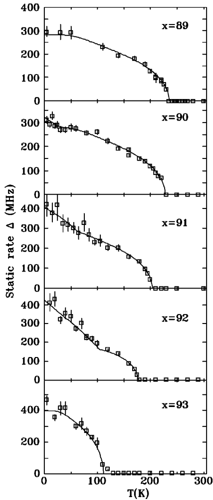
FIG. 3. Temperature dependence of the static relaxation rate ( \Delta ) showing the steady reduction in ordering temperature with increasing frustration and the effects of transverse spin freezing for 90 \geq x \geq 92 . Solid lines are fits to a modified Brillouin function with a linear term to include ordering of transverse spin components.
