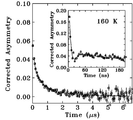
FIG. 1. Typical \mu SR signal, with fit, observed below T_c for a -Fe 92 Zr 8 . Inset shows the early-time region where the KT minimum characteristic of static order is visible. Note the clear separation in time-scales for the static and dynamic contributions.
