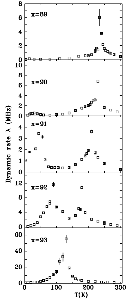
FIG. 2. Temperature dependence of the dynamic relaxation rate ( \lambda ) showing the high-temperature cusp ( T_c ) merging with the lower-temperature feature ( T_{xy} ) with increasing frustration.
