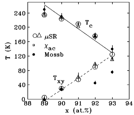
FIG. 4. Magnetic phase diagram for a - \text{Fe}_x\text{Zr}_{100-x} showing T_c and T_{xy} deduced from \mu SR data. Open circles mark values derived from the peak in \lambda , while the open triangles reflect values derived from fitting \Delta(T) . T_c 's derived from \chi_{ac} measurements on the same samples are also shown as small open squares. Values obtained on an independently prepared series of alloys and measured using applied-field Mössbauer spectroscopy are shown for comparison as solid symbols (Ref. 4).
