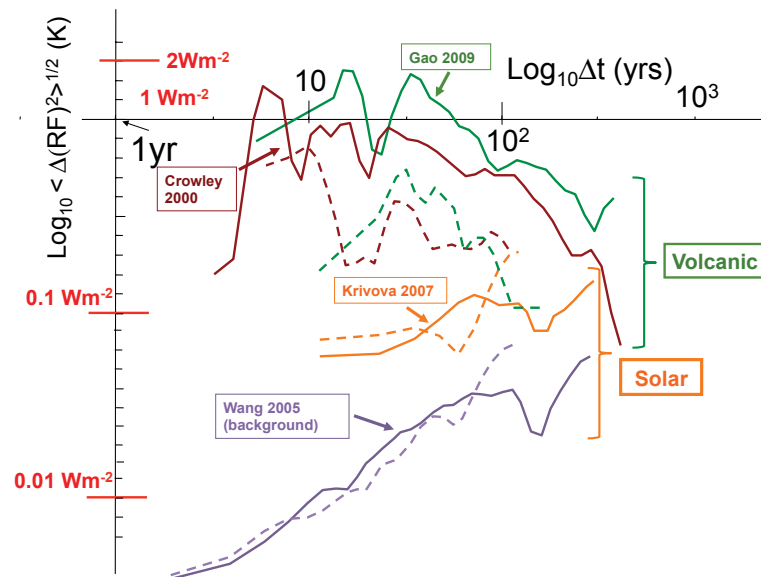
Fig. 9. Radiative forcings from various solar and volcanic reconstructions: a comparison of RMS Haar fluctuations for two solar and two volcanic radiative forcing reconstructions ( R_F ; units \text{Wm}^{-2} ). The dashed lines are for the period 1900–present, the solid lines for the period 1500–1900 (volcanic), 1610–1900 (solar). Note that the Wang et al. (2005) curve is only for the background solar forcing (without the 11 yr cycle) whereas the Krivova et al. (2007) curve has a 10 yr resolution. The volcanic series were from reconstructions of stratospheric sulfates using ice core proxies. All the structure functions have been increased by a factor of 2 so that they are roughly “calibrated” with the difference ( H > 0 ) and tendency ( H < 0 ) fluctuations; see Table 4. The basic forcings have roughly the same scaling properties in the industrial and preindustrial period, only the amplitudes of the volcanic forcings are slightly weaker in the recent epoch.
