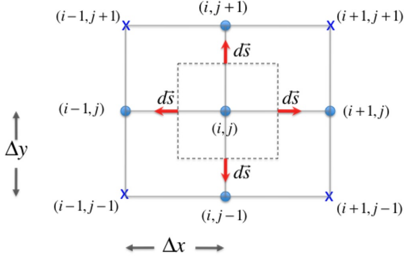
Figure B.1: Schematic of the uniform rectangular grid (solid lines) neighboring a pint (i, j) on the grid. The dashed box denotes the finite volume associated with the grid point (i, j) .
