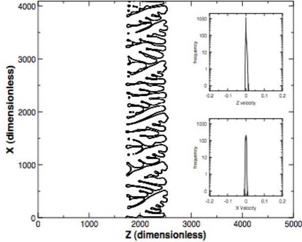
Figure 6.22: Directional solidification with the surface tension anisotropy oriented at 45^\circ with respect to the z -axis. Cooling parameters are the same as in Fig. 6.21. As the thermal gradient increases a competition between growth in the forward direction and the direction of surface tension anisotropy leads to multiple dendritic tip splittings, and a subsequent crystal structure that resembles seaweed. The insets show the velocity distribution in the x and z directions, respectively
