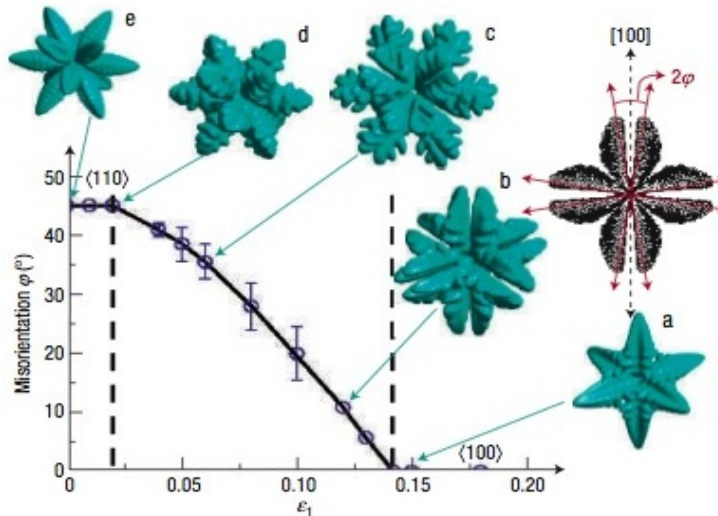
Figure 6.23: Figures (a)-(e) show the dendritic growth forms versus \epsilon_1 for \epsilon_2 = -0.02 . The azimuthal mis-orientation between branches changes continuously \Phi = 0 to \Phi = 45^\circ . The top right figure shows the interface cross sections at equal time intervals along a \langle 100 \rangle plane of sub-image (b). Projected contours show the mis-orientation between growth directions, quantified by the azimuthal angle \Phi . Reproduced from Ref. [89].
