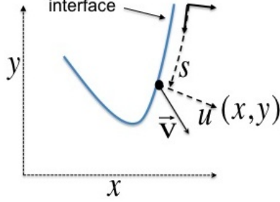
Figure A.1: Schematic of the (u, s) co-ordinates relative to an orthogonal co-ordinate system anchored onto the interface. The co-ordinate u measures distances normal to the interface while s measure the arclength long the interface. The vector \vec{v} denotes the velocity of the interface at the point indicated by the dot, which is situated at co-ordinates (0, s) . See also Fig. (C.1) for further details.
