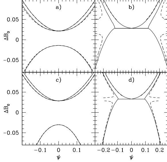
Figure 9.1: Phase diagrams in two (a,b) and three (c,d) dimensions. In all figures the parameters are t = 0.6 , v = 1 , u = 4 , B^\ell = B_0^\ell - 1.8\psi^2 (i.e., B_1^\ell = 0 , B_2^\ell = -1.8 ), B^x = 1 . The parameter w is 0.088 in (a) and (c), and 0.008 in (b) and (d). The solid lines are exact one-mode solutions and the dashed lines are approximate solutions as described by Eqns. (9.24) and (9.33).
