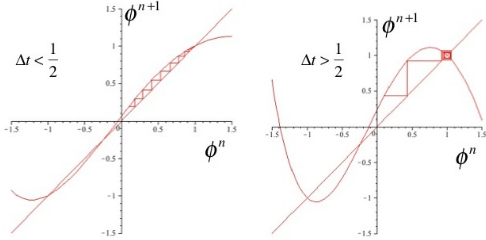
Figure B.2: Flow of iterates of the map \phi^{n+1} = f(\phi^n) where f(x) = x + \Delta t(x - x^3 - \hat{\lambda}U(1 - x^2)^2) . (Left) for \Delta t < 1/2 , iterates \phi^{n+1}(i) flow to the fixed point \phi^* = 1 . (Right) For \Delta t > 1/2 the fixed point generates a so-called limit cycle. Further increasing \Delta t will cause the iterates \phi^{n+1}(i) to diverge. In this figure \hat{\lambda}U = -0.25 .
